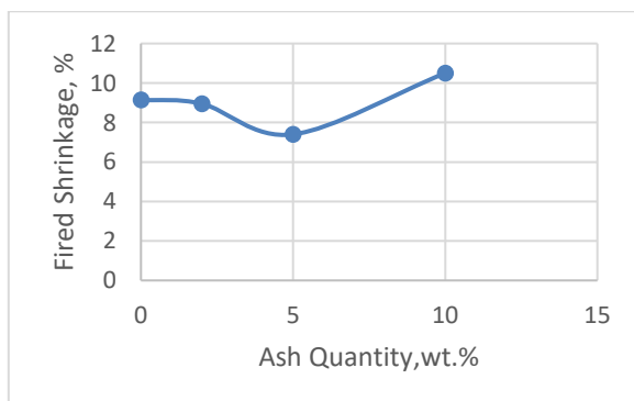
Figure 1. Fired shrinkage- ash wt.%
