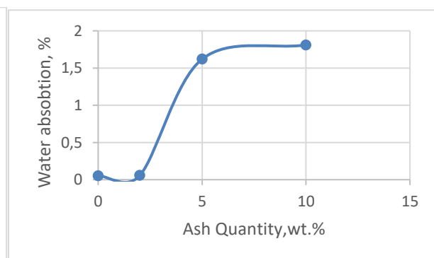
Figure 2. Water absorption-ash wt.%
